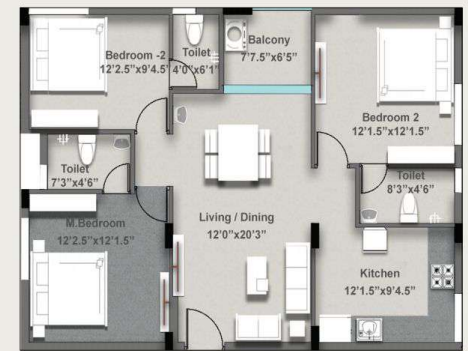
2nd - 5th FLOOR
